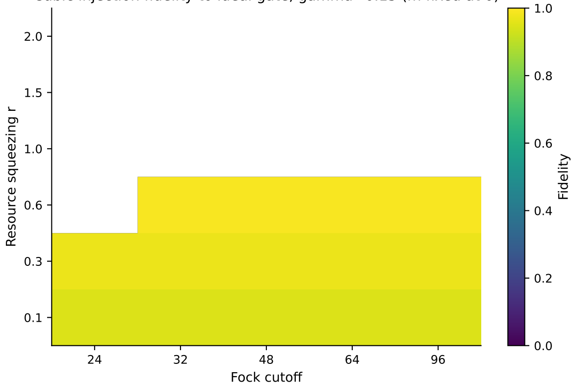
Cubic injection fidelity to ideal gate, gamma=0.15 (m fixed at 0)
