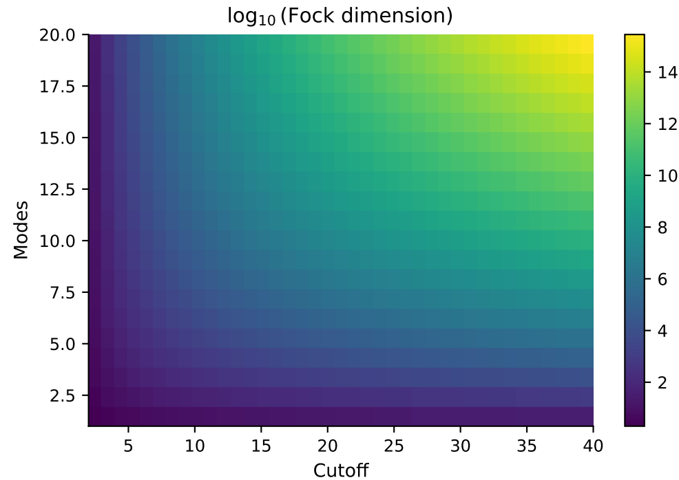
Fock-space dimension and memory scaling ( D = \text{binom}(\text{modes} + \text{cutoff} - 1, \text{modes}) )
