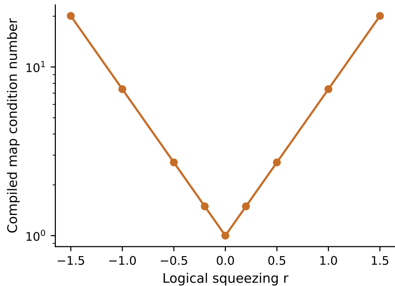
Squeezing gate compilation, resource squeezing r=1.2
