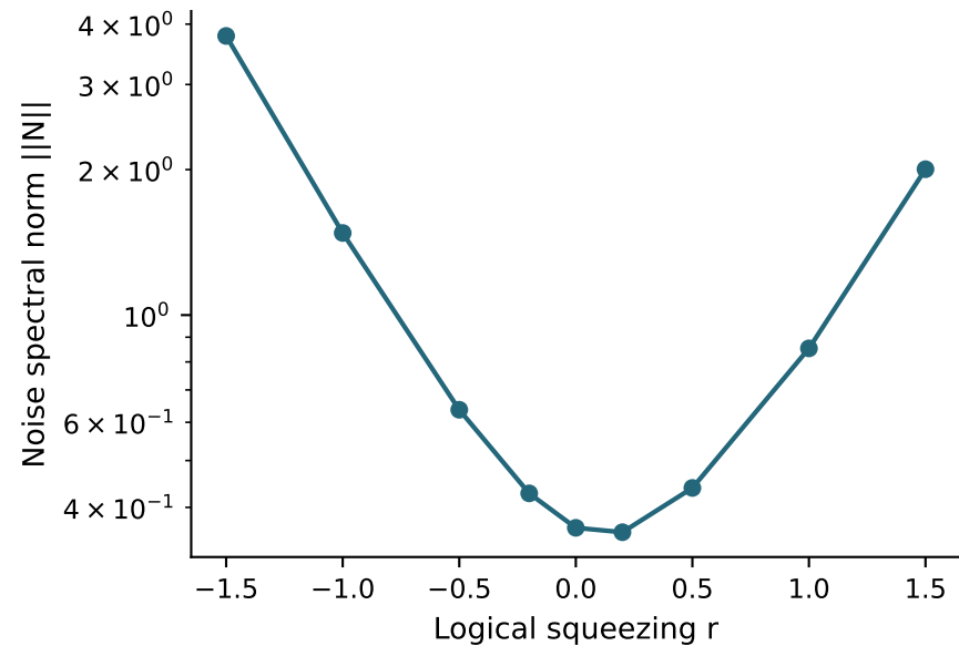
Squeezing gate compilation, resource squeezing r=1.2
