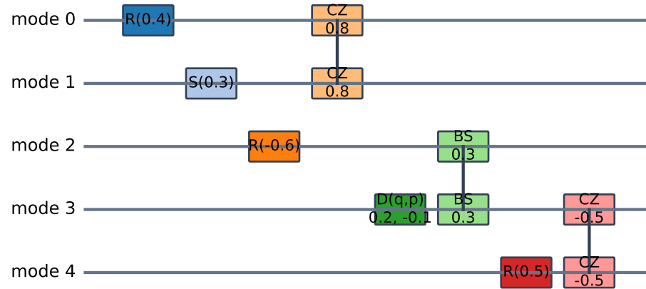
Photonic circuit
