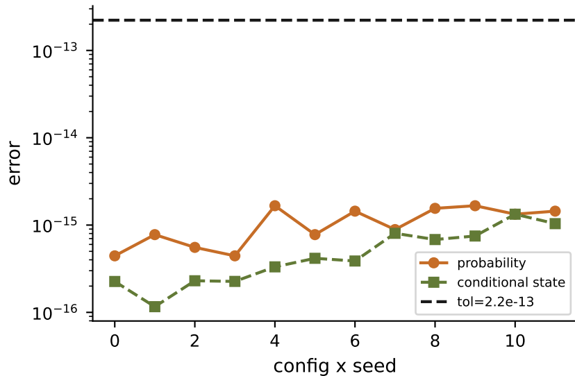
Branch agreement vs. MentPy projection
