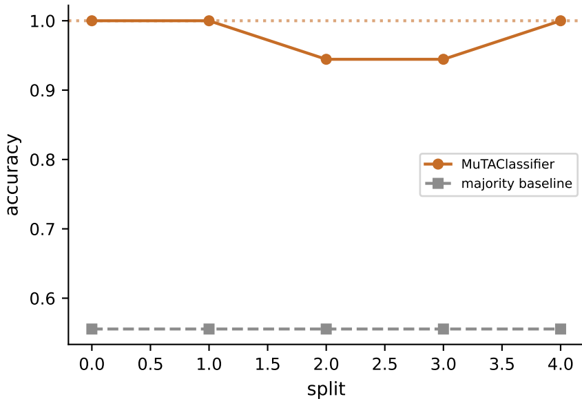
Held-out accuracy per split
