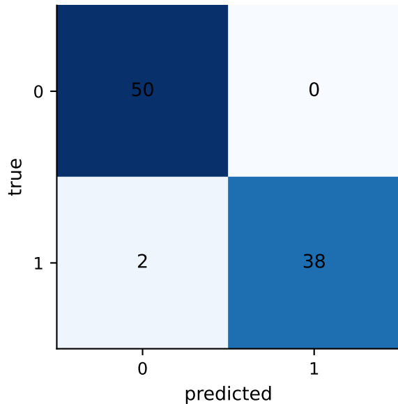
Aggregated confusion matrix
