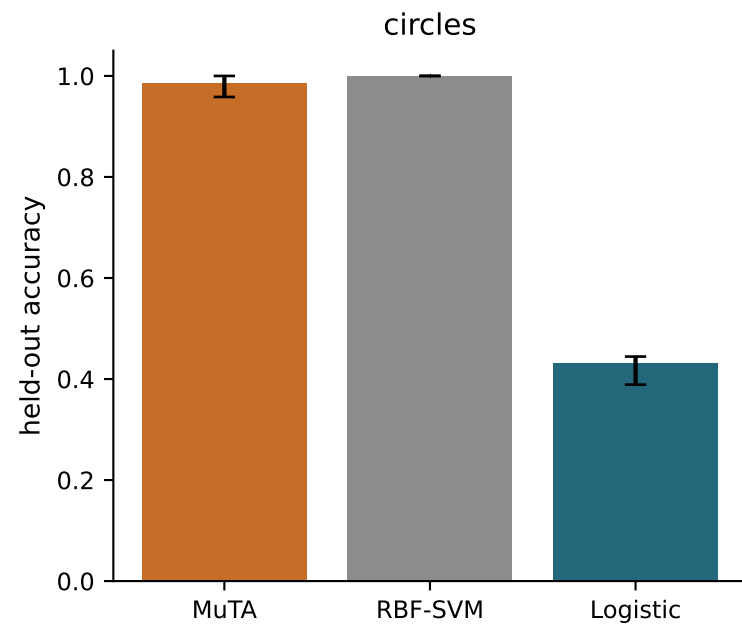
R27: kernel classification, median +/- 95% bootstrap CI, 8 seeds (structural=pass; outcome=descriptive)
