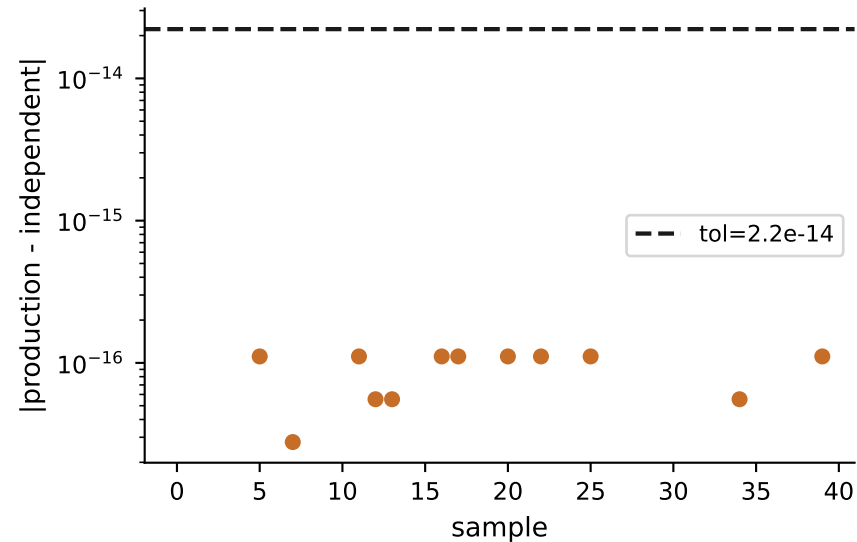
Random-state agreement
