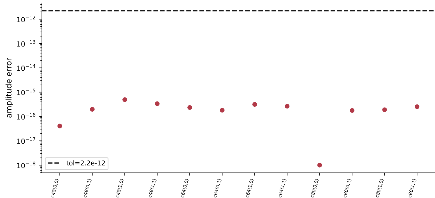
R40: raw Piquasso CZ vs. production dispatch (status=pass)
