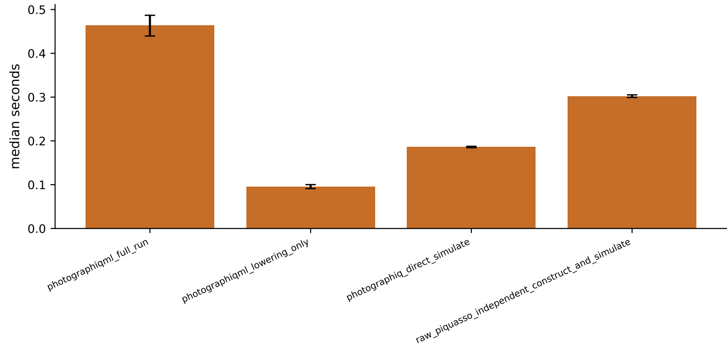
R42: abstraction overhead, matched 1-wire workload (wrapper overhead=0.182s)
