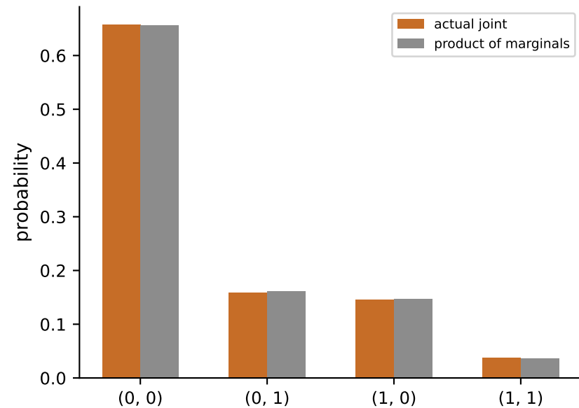
Joint vs. product of marginals (TV=0.0030)
