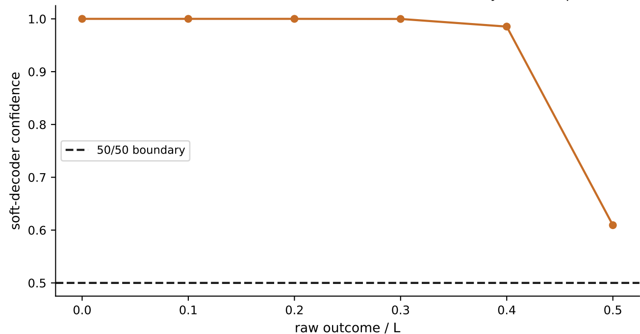
R46: soft-decoder calibration, ideal site \rightarrow cell boundary (status=pass)
