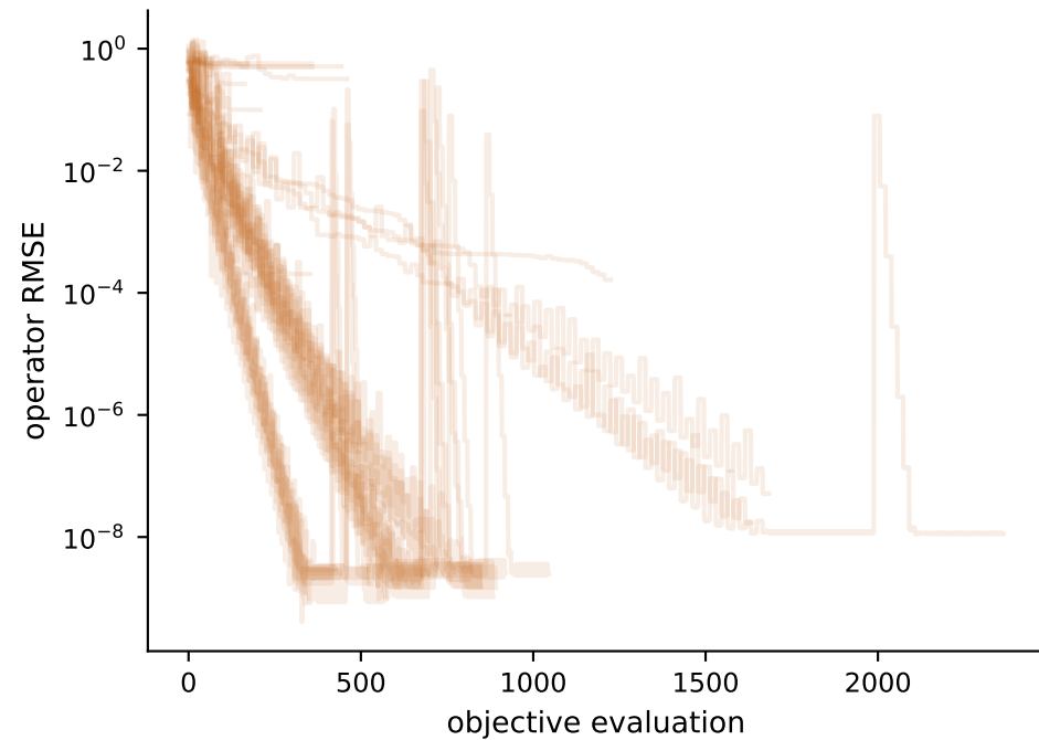
All optimization traces
