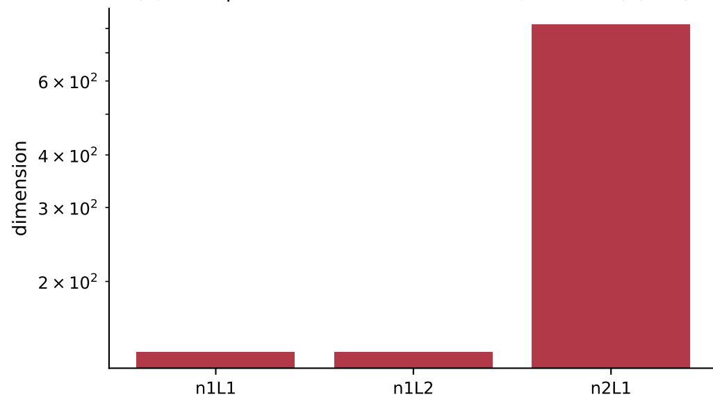
(b) Total-photon Fock dimension D=C(K+m-1,m) (R36)
