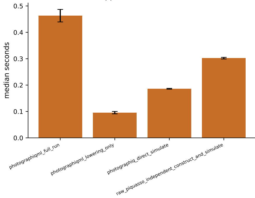
(c) Abstraction overhead, matched 1-wire workload (R42) wrapper overhead=0.182s
