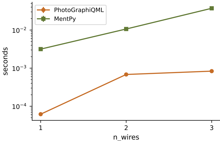
Matched-workload runtime (median +/- IQR/2)
