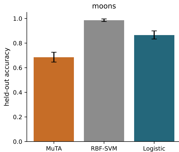
R27: kernel classification, median +/- 95% bootstrap CI, 8 seeds (status=pass)
