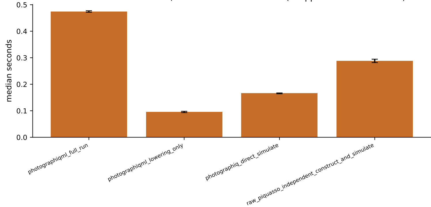
R42: abstraction overhead, matched 1-wire workload (wrapper overhead=0.213s)
