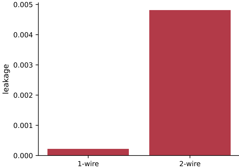
Max marginal code-subspace leakage
