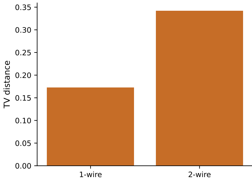
Decoded TV distance from ideal logical target
