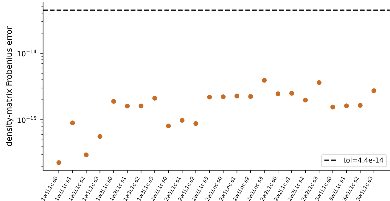
R5: independent brute-force contraction vs. MuTA.run (status=pass)
