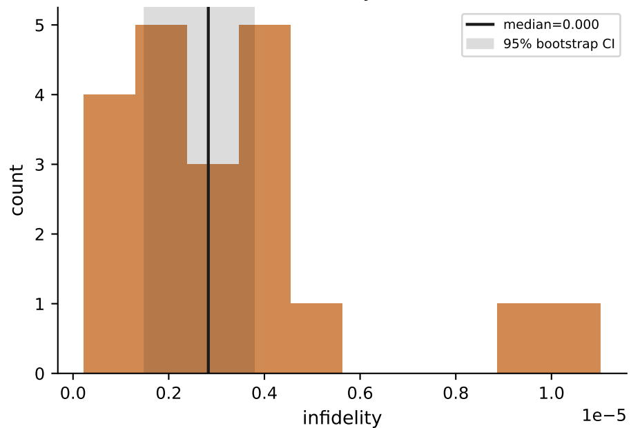
Final test-infidelity distribution
