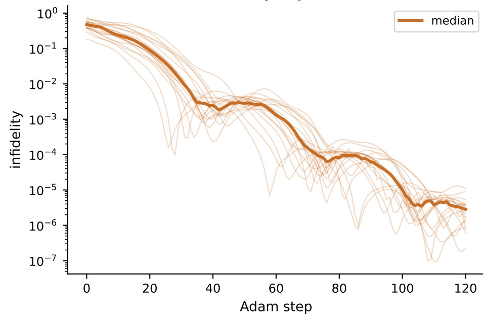
Held-out test infidelity trajectories (20 seeds)
