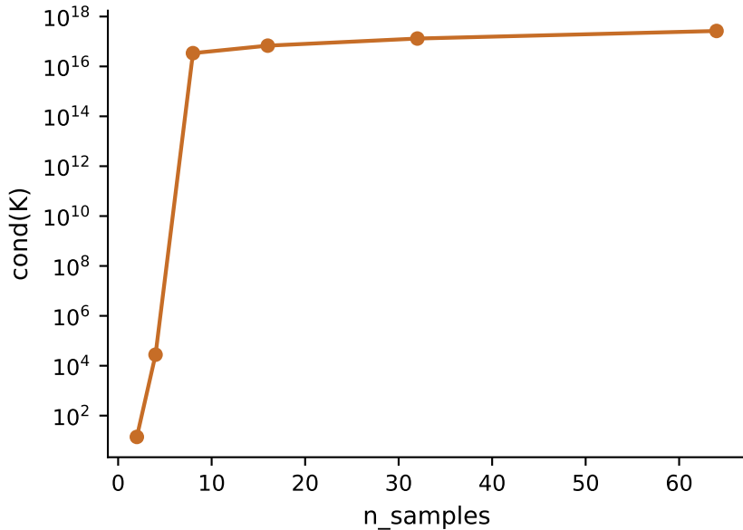
Gram-matrix condition number
