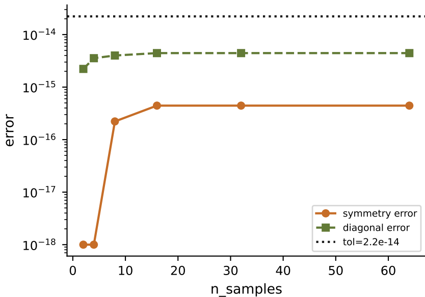
Symmetry / unit-diagonal error
