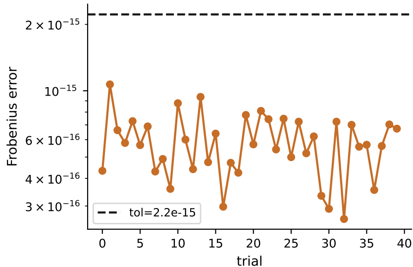
Full 3-angle Euler sequence
