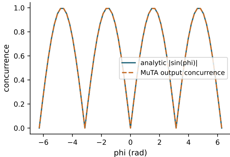
Induced concurrence
