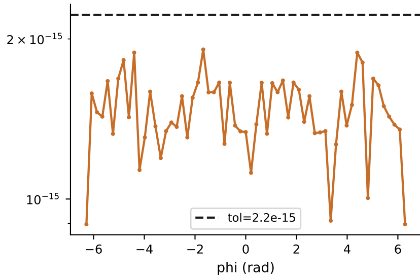
\exp(i\phi XX/2) Frobenius error
