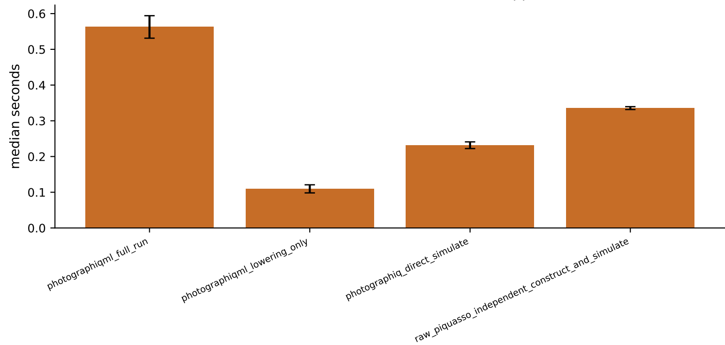
R42: abstraction overhead, matched 1-wire workload (wrapper overhead=0.222s)
