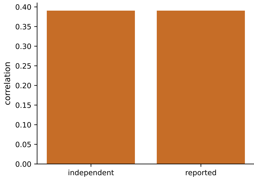
\langle Z_0 Z_1 \rangle connected correlation (error=0.00e+00)
