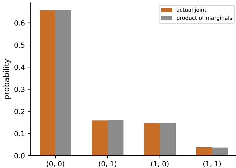
Joint vs. product of marginals (TV=0.0030)
