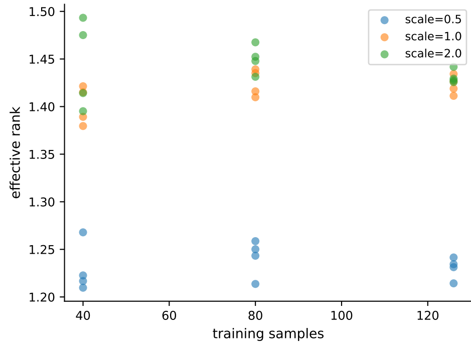
Kernel spectrum
