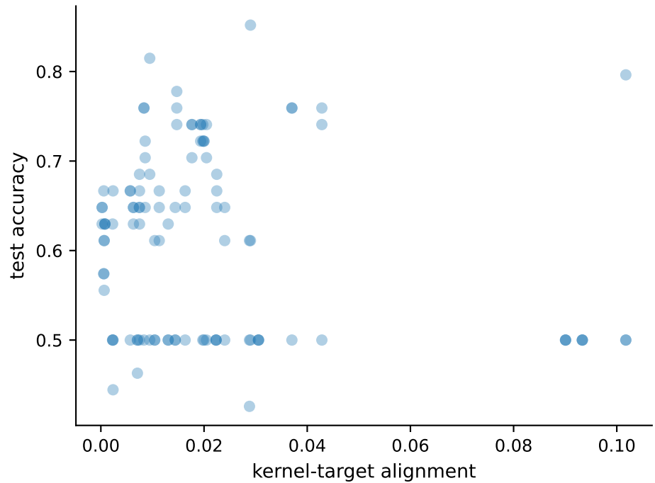
Performance ablation
