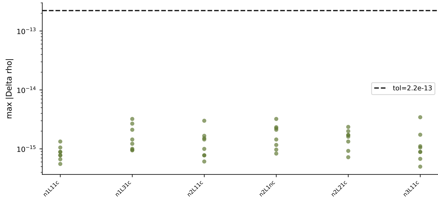
R9: MuTA vs. MentPy density-matrix agreement (status=pass)
