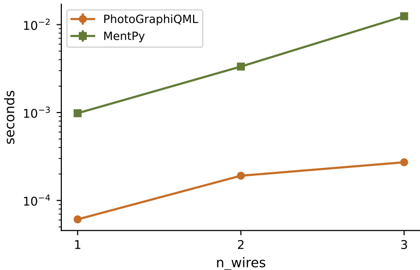
Matched-workload runtime (median \pm IQR/2)
