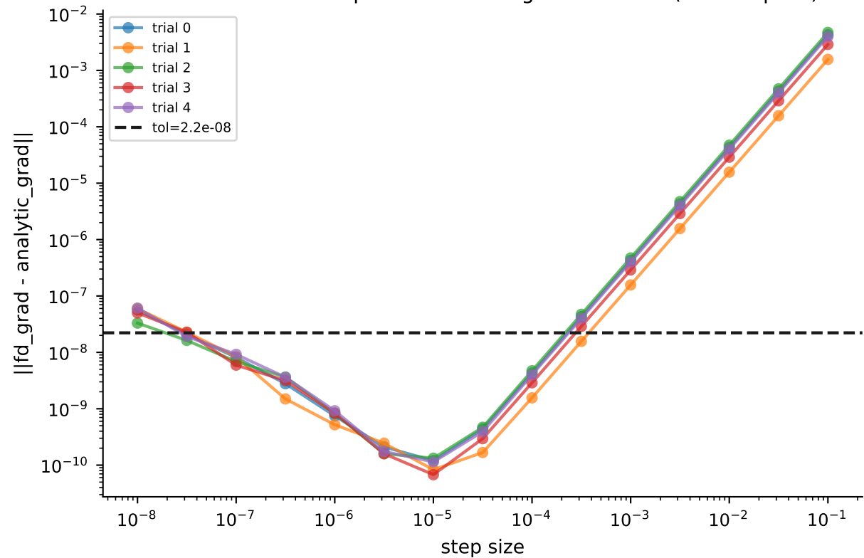
R18: central-FD vs. parameter-shift gradient error (status=pass)
