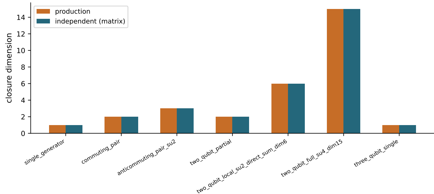
R32: Lie-closure dimension agreement (status=pass)
