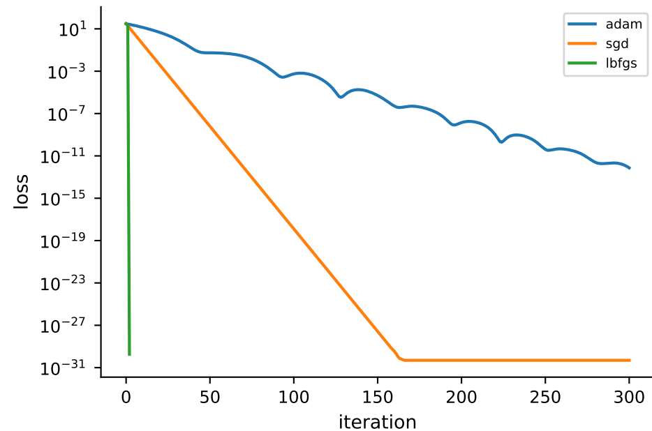
Quadratic bowl
