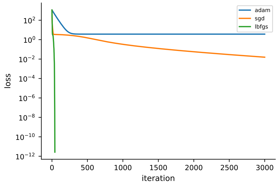
Rosenbrock
