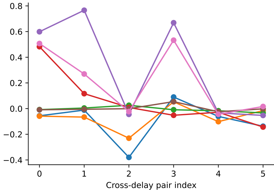
Degree-two cross target test R^2
