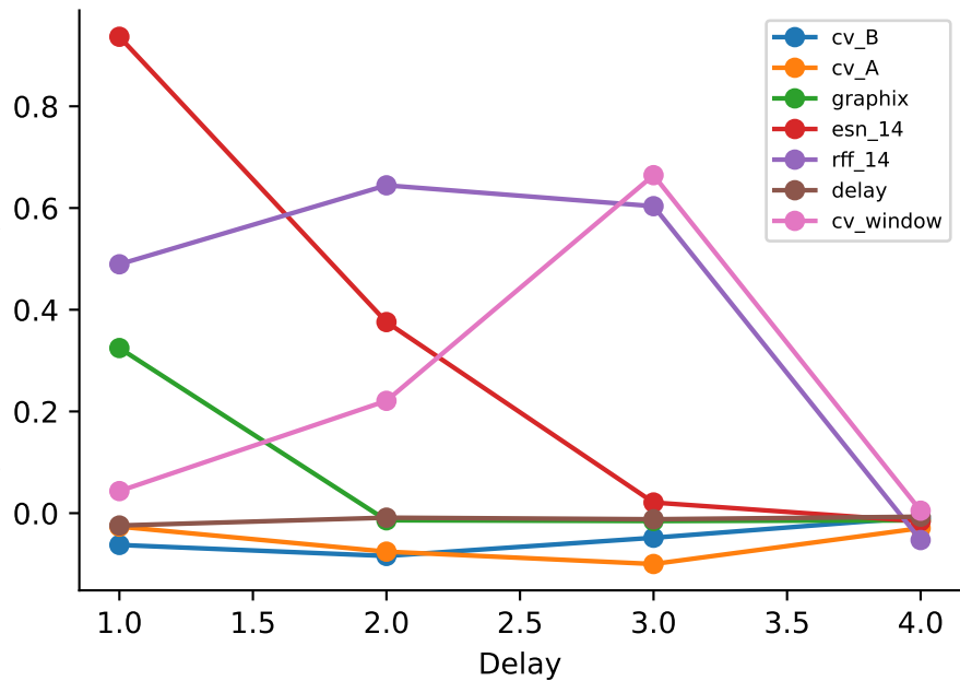
Degree-two self target test R^2
