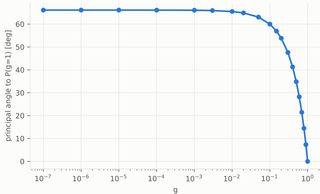
g rotates the feature, not only its amplitude
