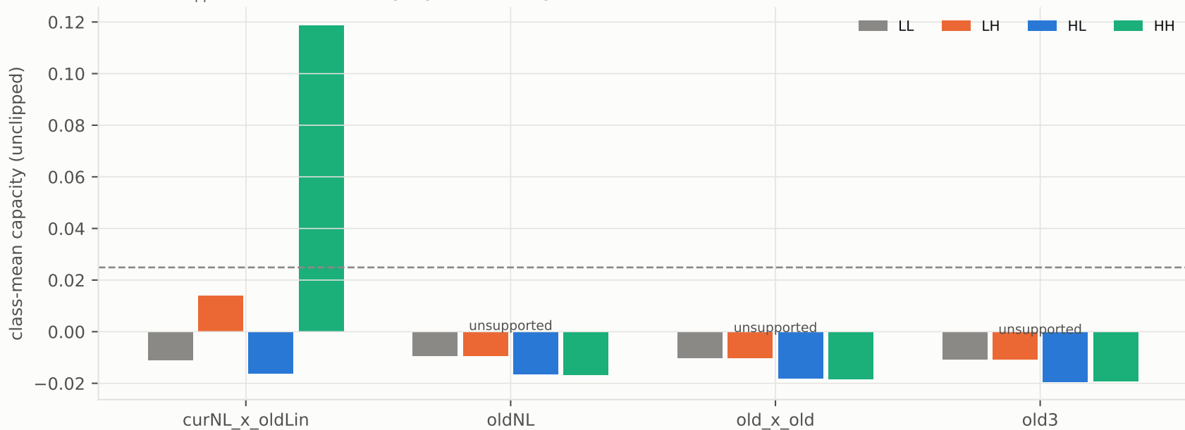
Combined nonlinear memory by class: only current-NL \times old-linear is reachable
