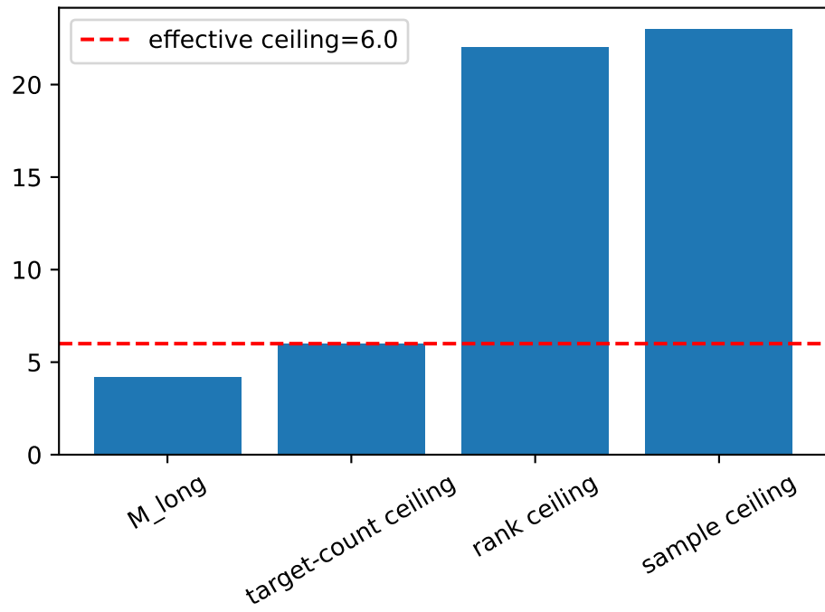
Capacity-ceiling diagnostic (fraction=69.51%, contaminated=False)
