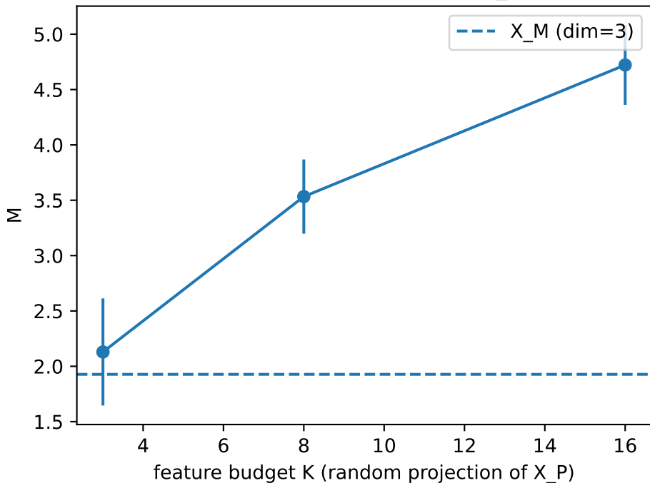
FAST mode: M vs feature budget (n_repeats=3)
