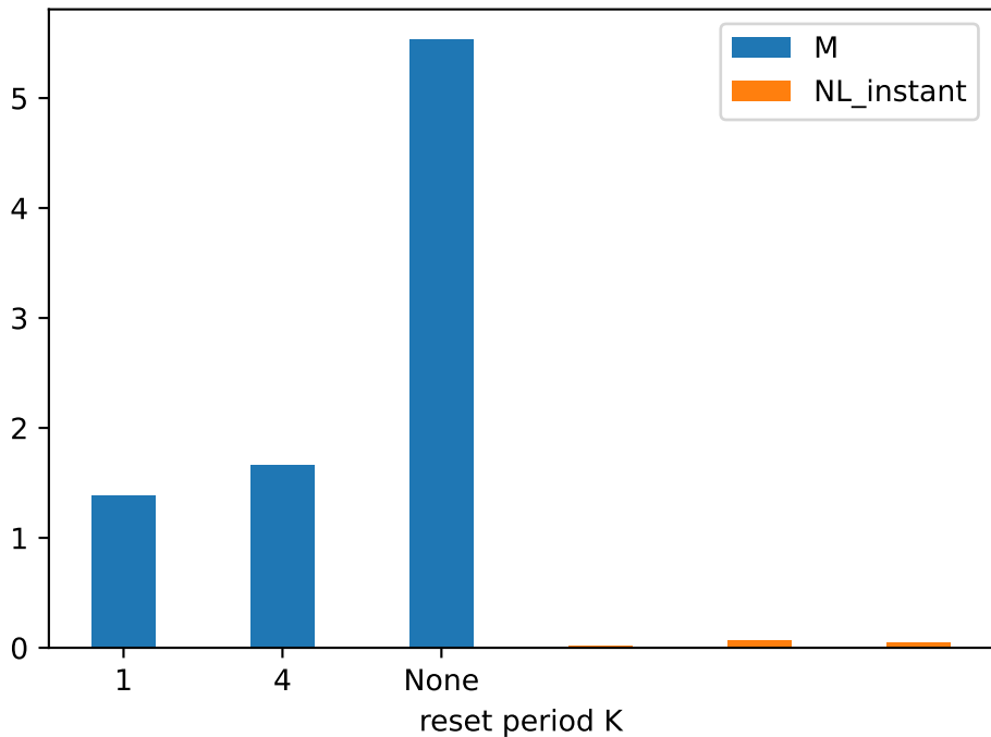
FAST mode: persistence/reset ablation, 1 seed
