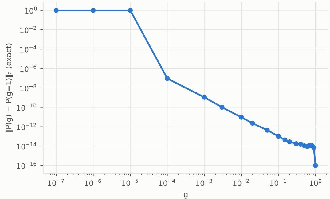
The accessible nonlinear subspace is identical for all g \geq 1e-4
