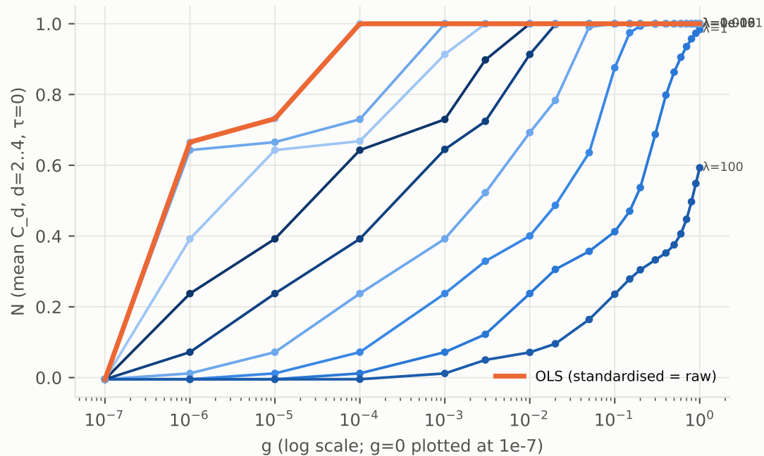
Only the ridge penalty grades N(g) ; OLS is a step at g \approx 0
