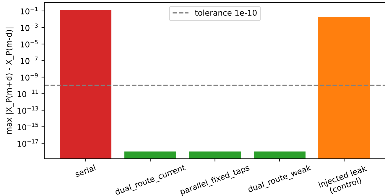
Structural isolation -- SMOKE, 1 realization, exact features (atol=1e-10)
