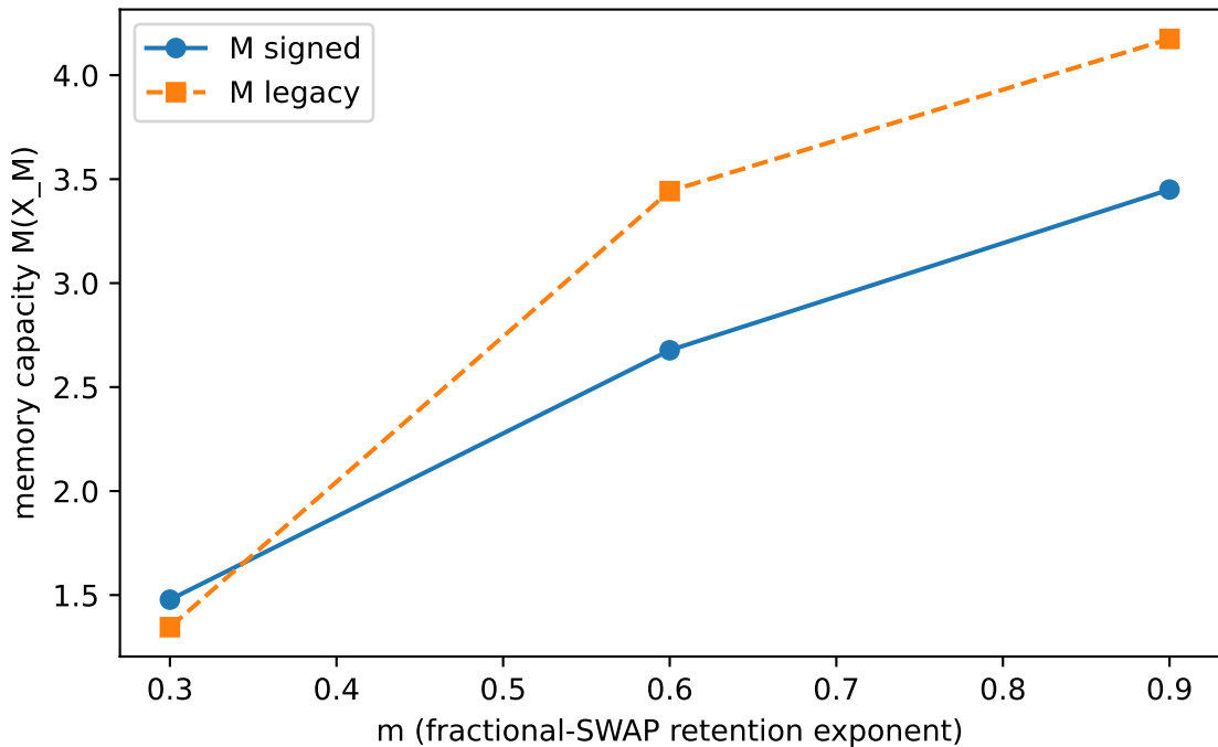
Memory capacity vs m -- SMOKE, 1 reservoir seed, signed bias-corrected
