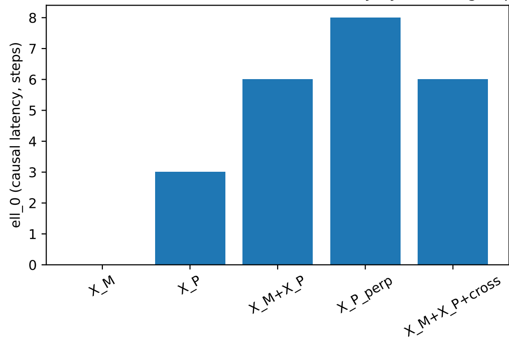
DISCOVERY mode, 1 seed: causal latency by feature group
