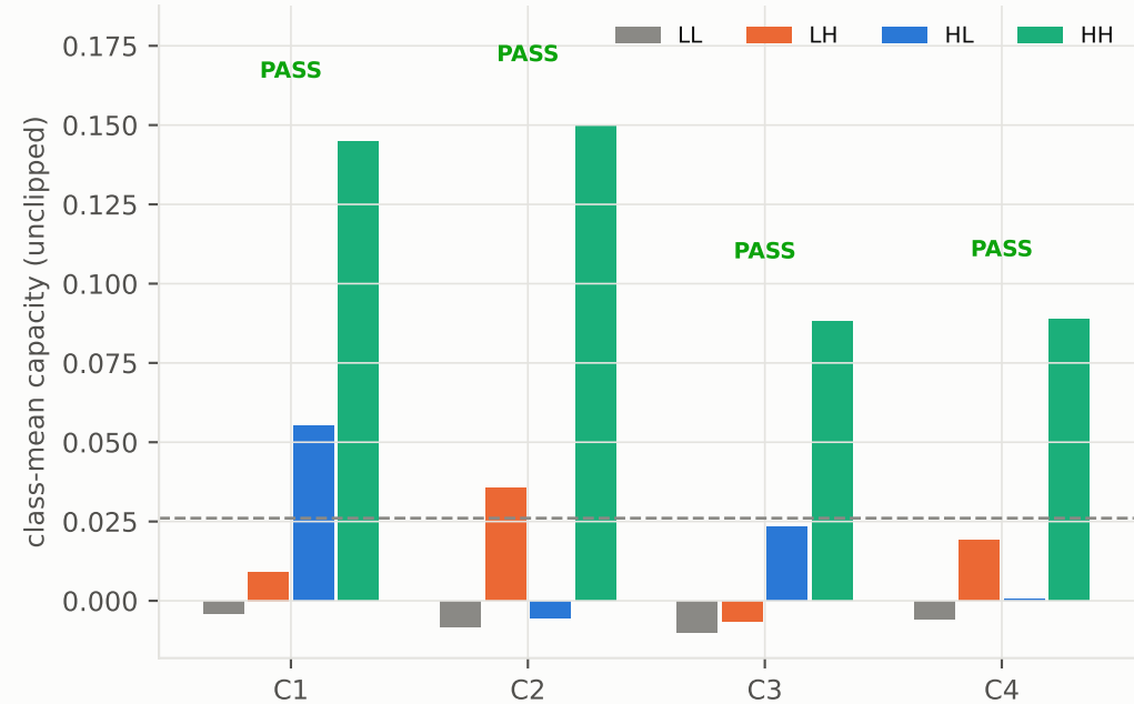
quadrant means — ridge
