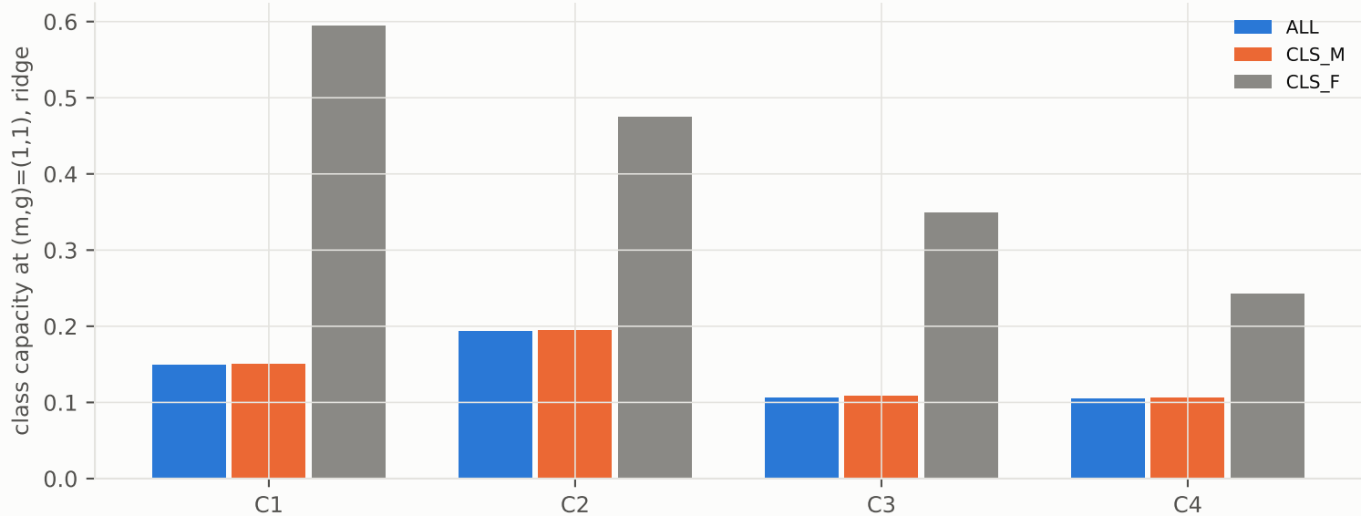
Quantum operational readout vs classical products of marginals
