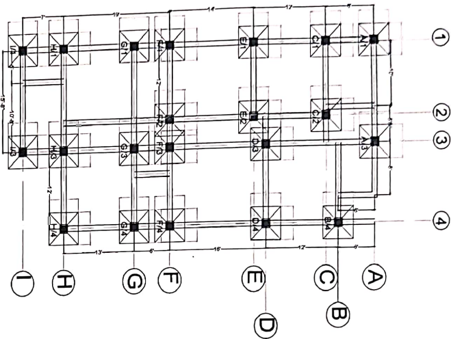
FOUNDATION PLAN
