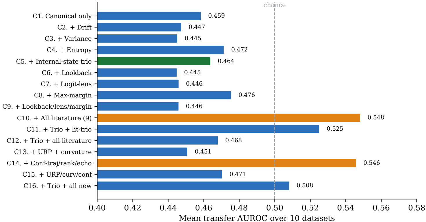
GPT-J-6B: detection AUROC by feature configuration
