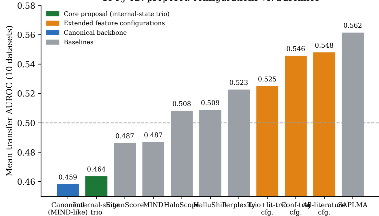
GPT-J-6B: proposed configurations vs. baselines
