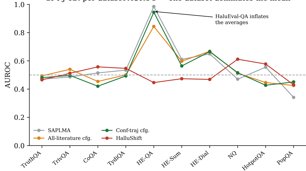
GPT-J-6B: per-dataset AUROC — one dataset dominates the mean
