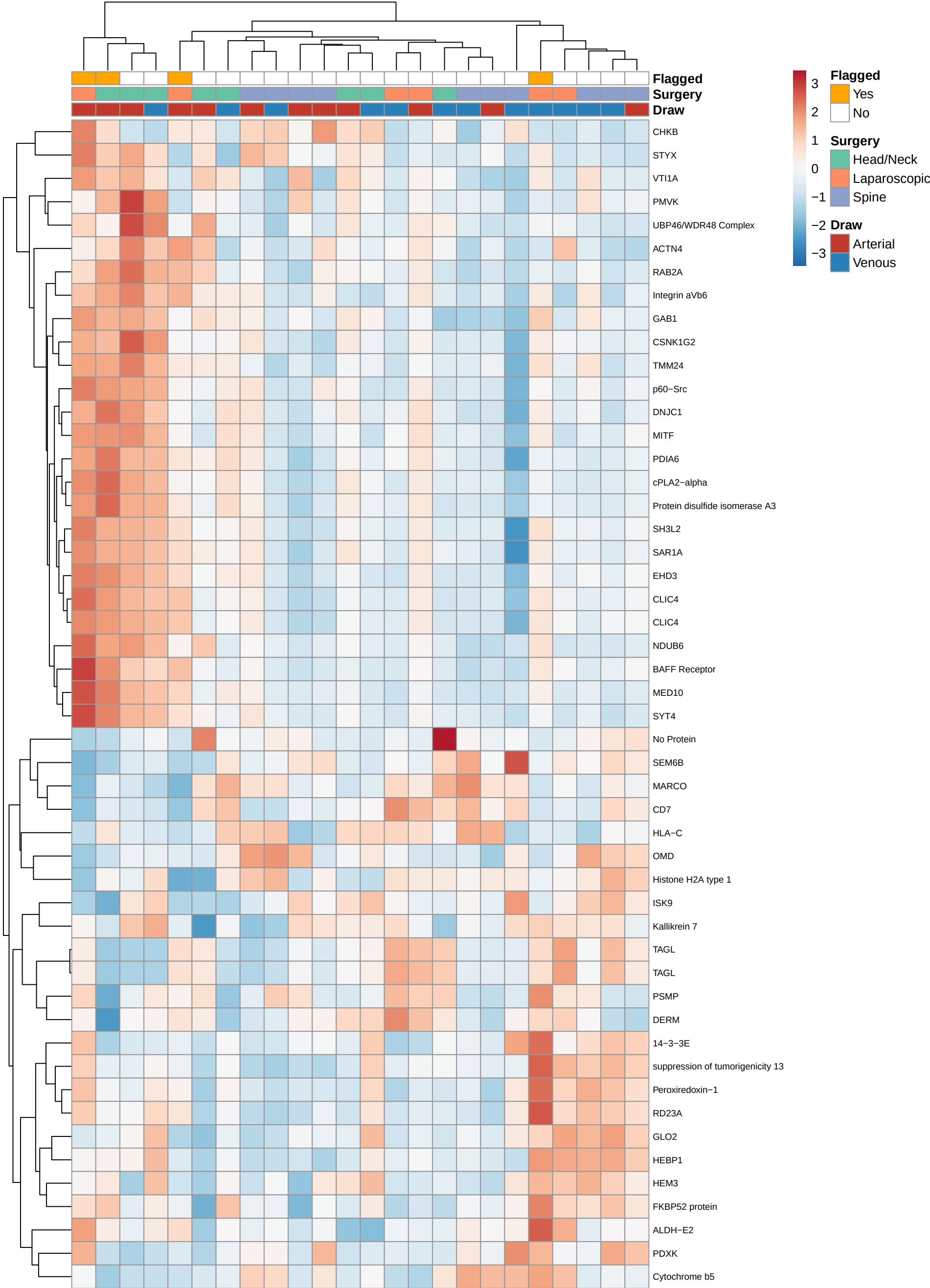
Top 50 A-V proteins (row-scaled log2 RFU)
