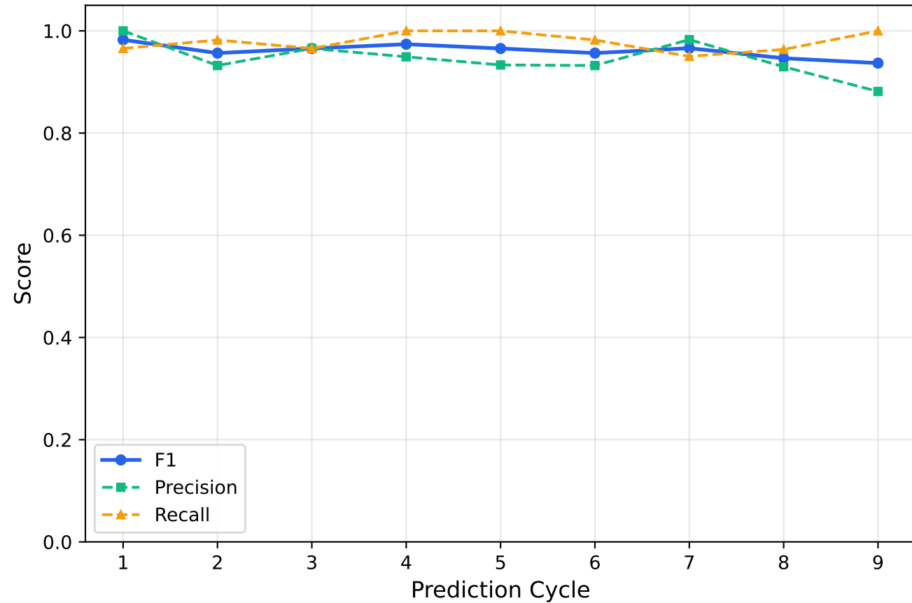
NYC 311 — Metric Convergence
