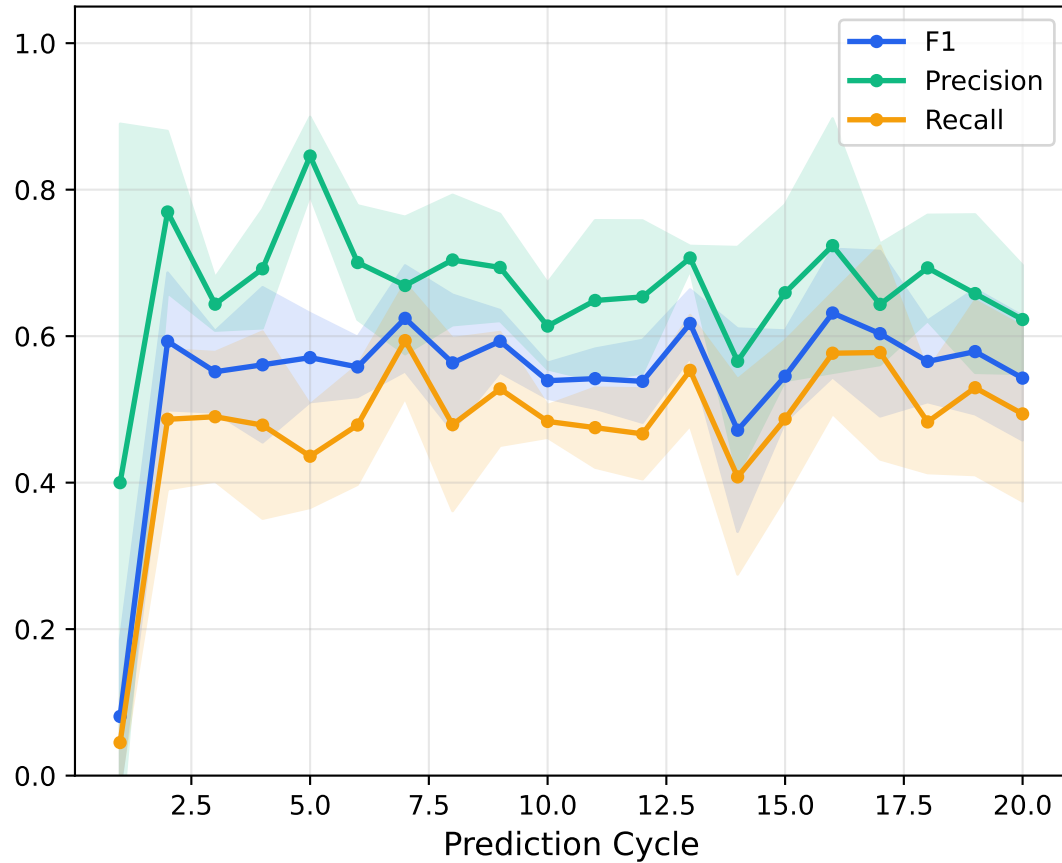
Metric Convergence (mean \pm std)
