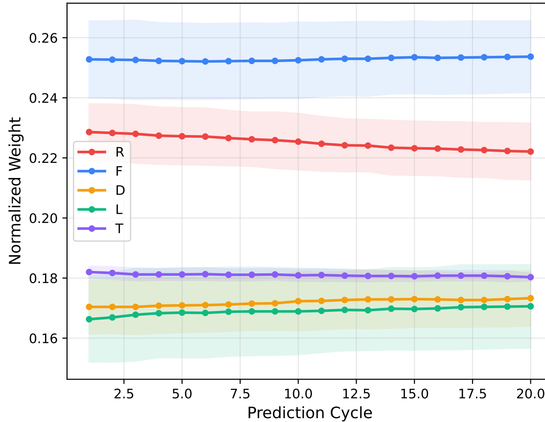
Weight Evolution (mean \pm std)
